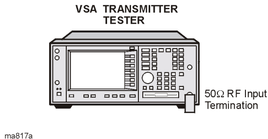
DANL/Noise Figure Test Setup
